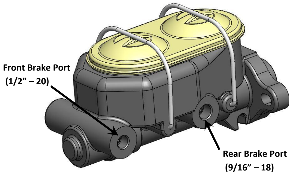
Figure 1 - Brake Line Orientation
