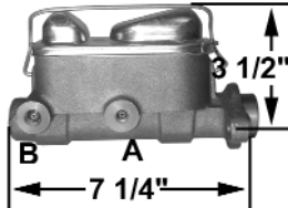
MC1001PZ Remote fill $139.95 Use for disc/drum Outlets: A 1/2-20 B 9/16-18 Bore size: 1" Ports: left Shallow piston hole power brakes
