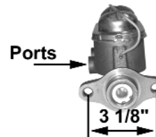
MC11680M $89.95 Use for disc/drum Outlets: A 1/2-20 B 7/16-24 Bore size: 15/16" Ports: left Deep piston hole manual brakes
