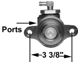
MC1001PZ Remote fill $139.95 Use for disc/drum Outlets: A 1/2-20 B 9/16-18 Bore size: 1" Ports: left Shallow piston hole power brakes
