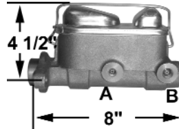
MC1001MZ Remote fill $139.95 Use for disc/drum Outlets: A 1/2-20 B 9/16-18 Bore size: 1" Ports: left Deep piston hole manual brakes
