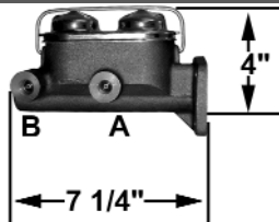
MC11897P/M $119.95 Use for disc/disc Outlets: A 1/2-20 B 7/16-24 Bore size: 1 1/8" Ports: right Deep piston hole power brakes
