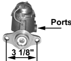
MC11897P/M $119.95 Use for disc/disc Outlets: A 1/2-20 B 7/16-24 Bore size: 1 1/8" Ports: right Deep piston hole power brakes
