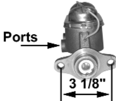
MC11378M $89.95 Use for disc/drum Outlets: A 3/8-24 B 1/2-20 Bore size: 1" Ports: left Deep piston hole manual brakes
