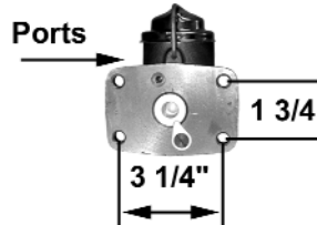
MC11323M $89.95 Use for drum/drum Outlets: A 1/2-20 B 9/16-20 Bore size: 1" Ports: left Deep piston hole manual brakes
