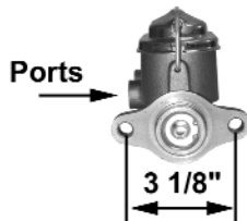
MC11488M $89.95 Use for drum/drum Outlets: A 1/2-20 B 9/16-18 Bore size: 1" Ports: left Deep piston hole manual brakes
