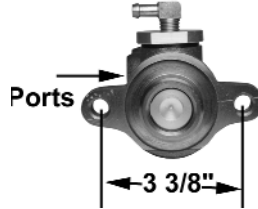
MC1001MZ Remote fill $139.95 Use for disc/drum Outlets: A 1/2-20 B 9/16-18 Bore size: 1" Ports: left Deep piston hole manual brakes
