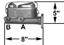
MC11680M $89.95 Use for disc/drum Outlets: A 1/2-20 B 7/16-24 Bore size: 15/16" Ports: left Deep piston hole manual brakes
