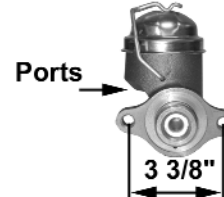
MC11268M Single outlet $89.95 Use for drum brakes only Outlets: 3/8-24 Bore size: 1" Ports: left & back Deep piston hole manual brakes
