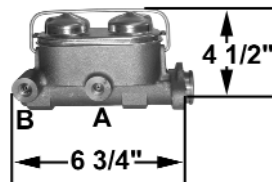
MC11378M $89.95 Use for disc/drum Outlets: A 3/8-24 B 1/2-20 Bore size: 1" Ports: left Deep piston hole manual brakes
