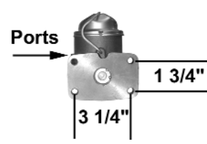
MC11571P/M $89.95 Use for disc/drum Outlets: A 1/2-20 B 9/16-20 Bore size: 1" Ports: left Deep piston hole manual brakes
