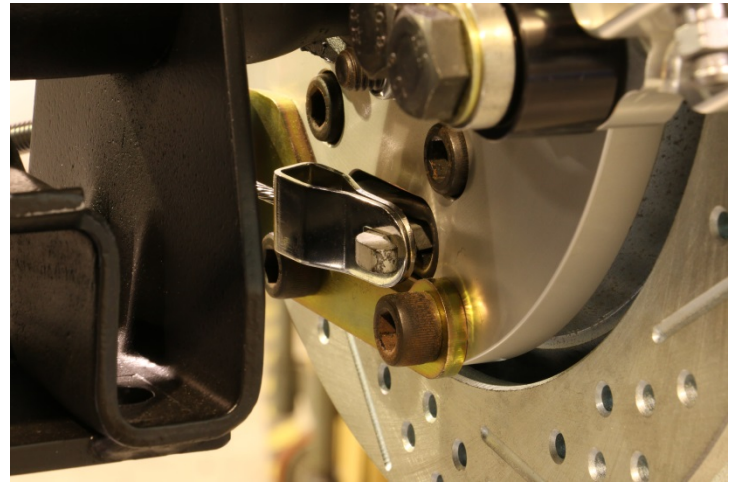
Figure 3 - Inner Wire Inserted and the Clevis Attached
